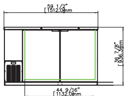
ABBC-58(G) Front
