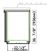
ABBC-Common View
