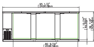
ABBC-94(G) Front
